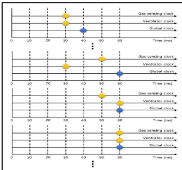
Fig. 13. Relative synchronization after 3 rd tick
